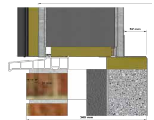
hup! on 300mm existing wall - on cill
