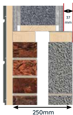
hup! on 250mm existing wall - full clad
