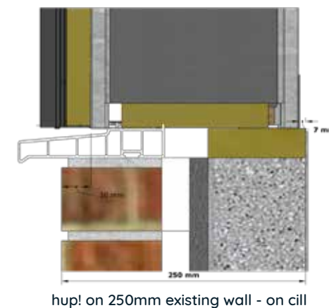
hup! on 250mm existing wall - on cill
